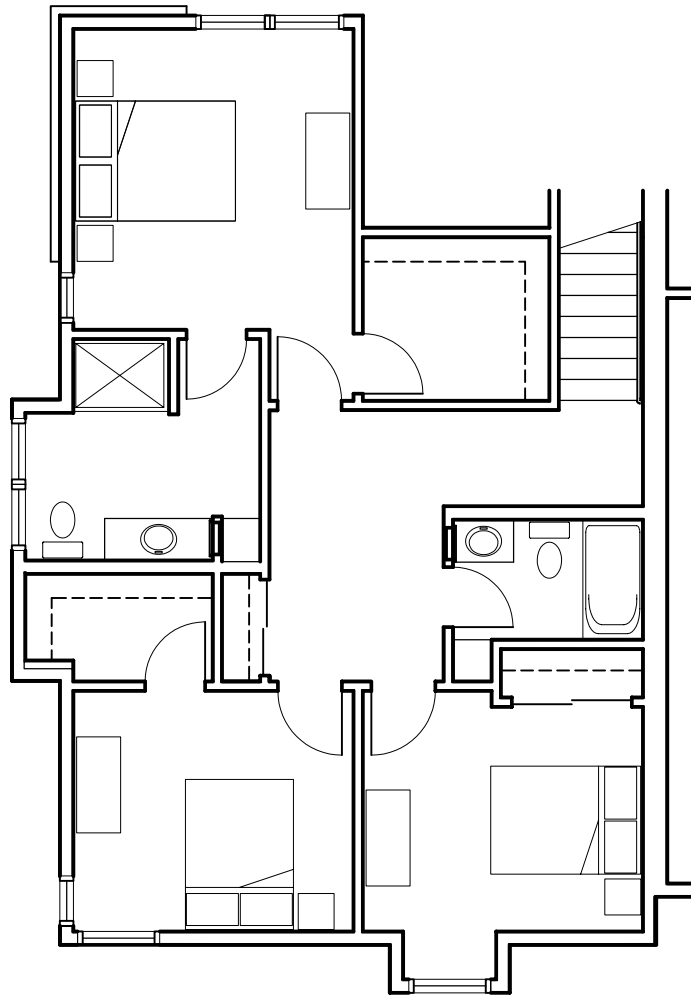
TOWNHOUSE END UNIT SECOND FLOOR: 789 SF
