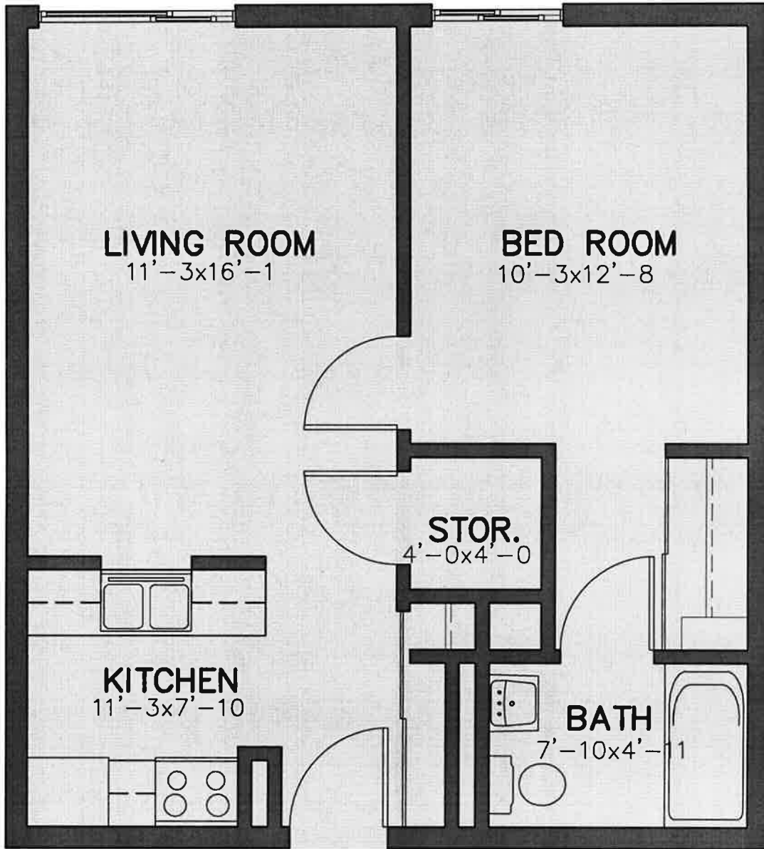
BURKE TYPE IIA SCALE : 1/4" = 1' 0"
