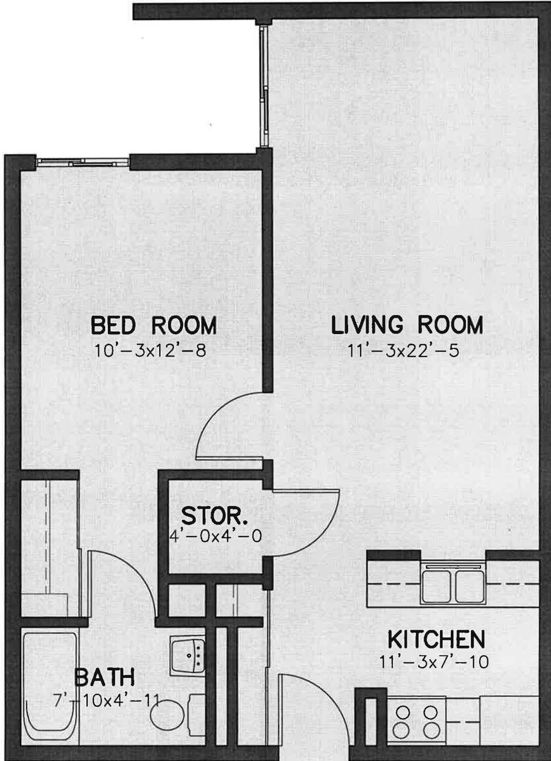
BURKE TYPE III SCALE : 1/4" = 1' 0"
